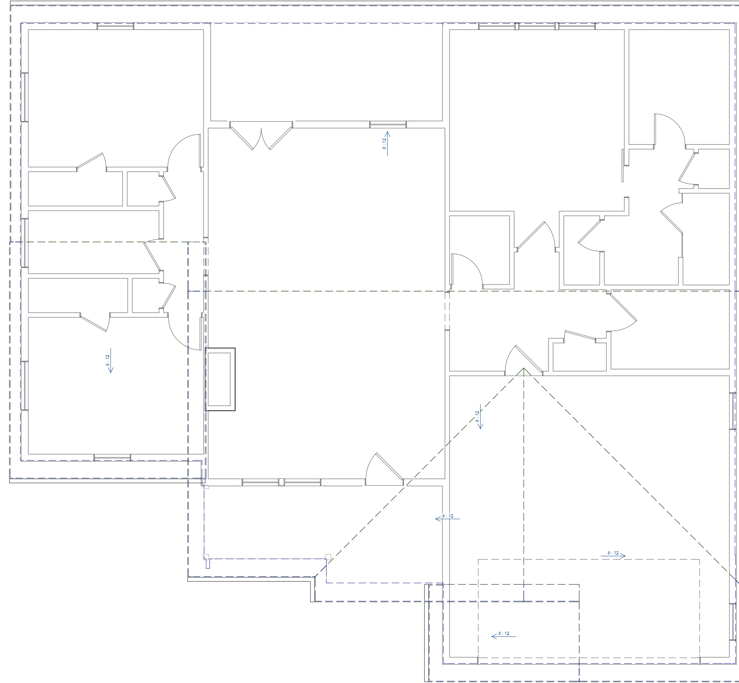
Roof Plan View
